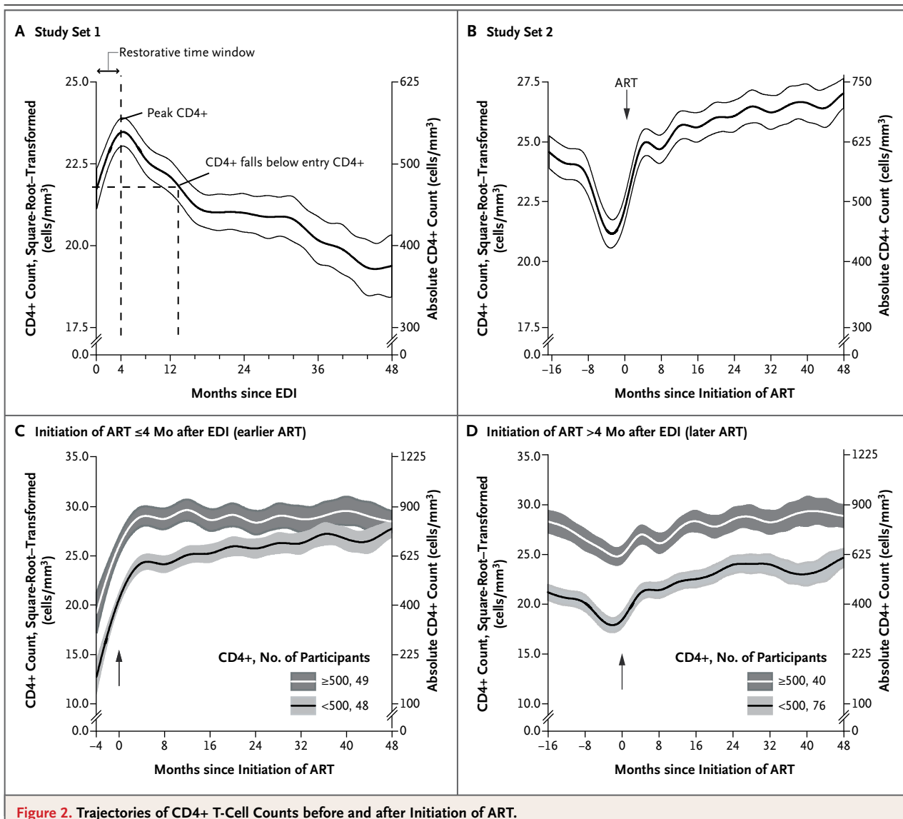
Figure 2. Trajectories of CD4+ T-Cell Counts before and after Initiation of ART.
